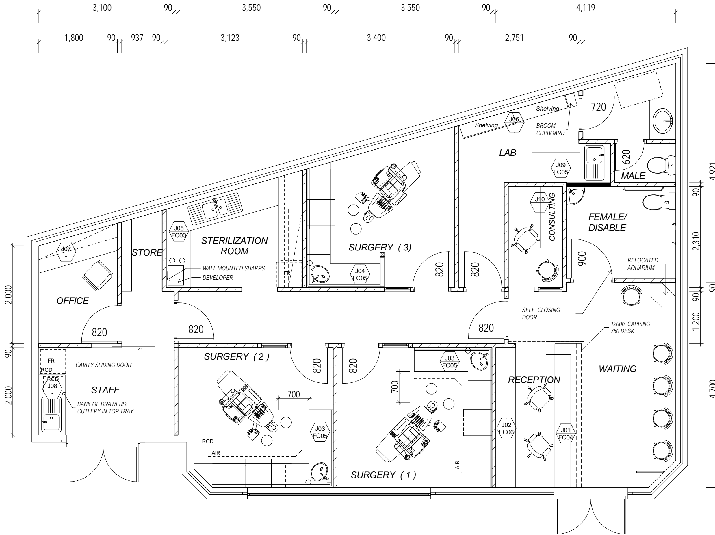
LAYOUT PLAN / PROPOSED DENTAL ROOMS SCALE 1:50
